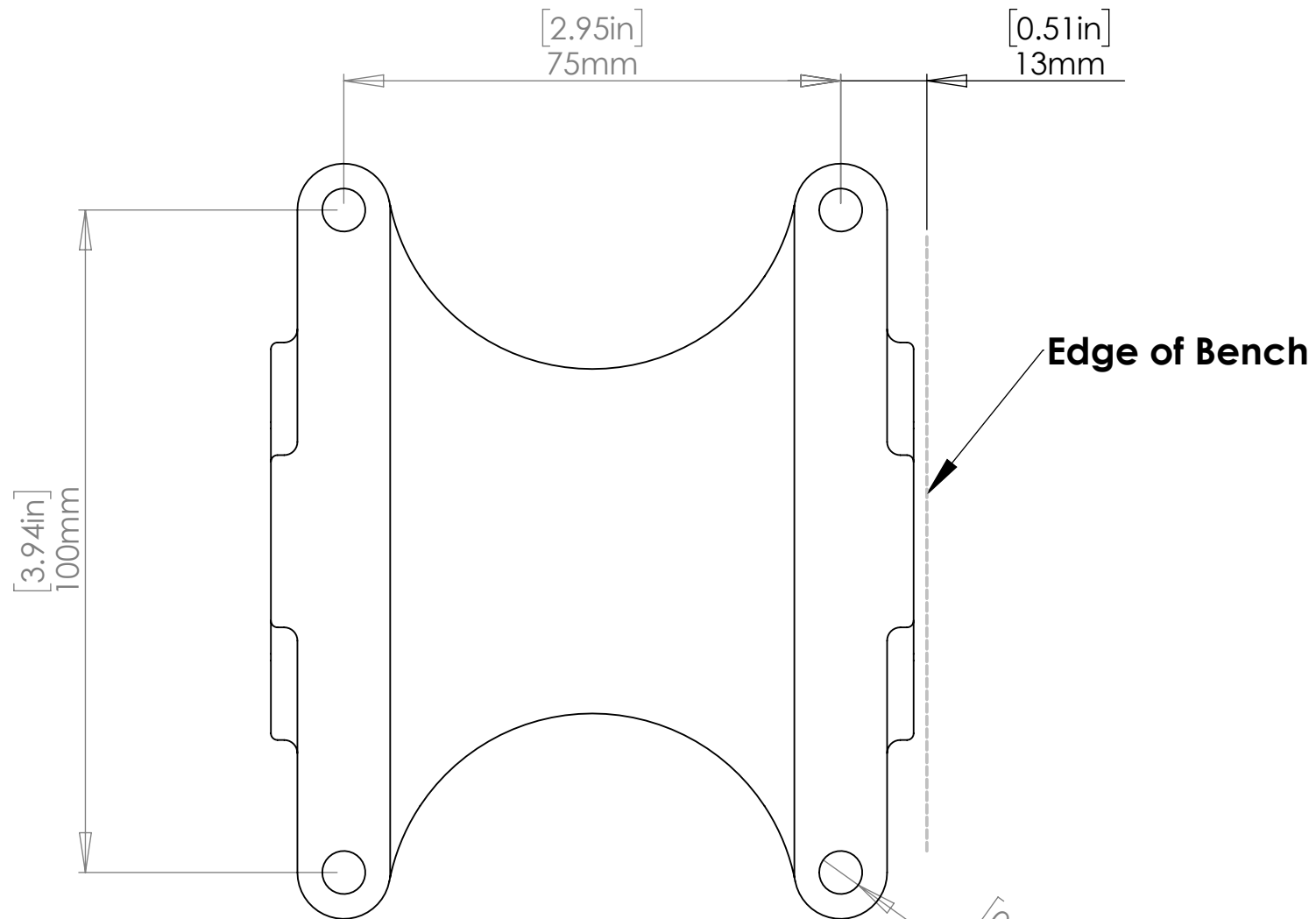
Agile 50 RM Hole positions for Bench Scale 1:1 Check sizes before use
